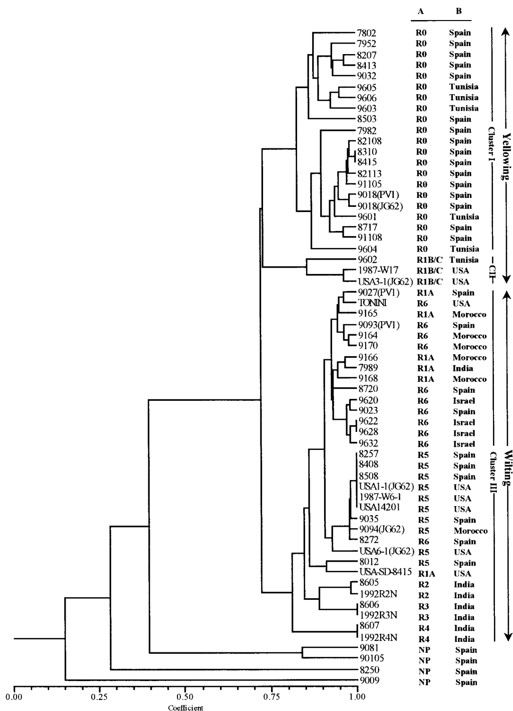
Figure 2. Dendrogram derived from RAPD analysis of 57 isolates F. oxysporum f. sp. ciceris and four isolates of nonpathogenic F. oxysporum using primers OPI-01, OPI-09, OPI-18, OPF-06, OPF-10, OPF-12, and OPF-16. The dendrogram was derived by UPGMA (unweighted paired group method with arithmetic averages). The bottom scale is the percentage of similarity by Jaccard's similarity coefficient. A , Race assignment of an isolate: R0 = race 0, R1A = race 1A, R1/B = race 1B/C, R2 = Race 2; R3 = race 3, R4 = race 4, R5 = race 5, R6 = race 6, NP = Nonpathogenic F. oxysporum . B , Geographic origin of isolates.
