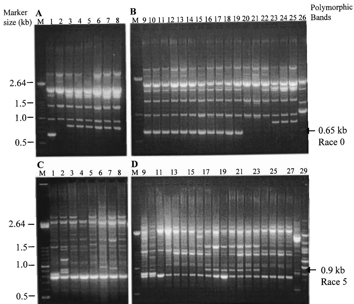
Figure 1. RAPDs generated by primer OPF-16 (A, B) and OPF-10 (C, D) using a DNA bulk of F. oxysporum f. sp. ciceris isolates of a race (A, C) and DNA from individual isolates representative of the race (B, D). DNA products were separated on a 1.5% agarose gel and stained with ethidium bromide. Numbers on the left side are the sizes of the 0.1-kb DNA ladder XIV (Boehringer-Mannheim) (lane M). Numbers on the right side are the sizes of the marker bands that identify races 0 (A and B) and 5 (C and D). A and C: lanes 1–8, DNA bulks for each of F. oxysporum f. sp. ciceris races 0, 1B/C, 1A, 2, 3, 4, 5, and 6. B: lanes 9–19, race 0 isolates Foc-7802, -9018 (JG62), -82108, -8717, -7952, -8207, -9032, -9601, -91118, -9604, -82118; lanes 20–22, race 1B/C isolates Foc-USA 3–1 (JG62), -1987 W-17, -9602; lanes 23–26, race 1A isolate Foc-7989, race 5 isolate Foc-8012, race 6 isolate Foc-9093 (PV1), and nonpathogenic F. oxysporum isolate Fo-9009, respectively. D: lanes 9–12, race 0 isolates Foc-7802, -91108, -9018 (JG62), -9601; lanes 13–16, race 1A isolates Foc-9027 (PV1), -9165, -9166, -7989; lanes 17–23, race 5 isolates Foc-8012, -8508, -9035, -USA 1–1 (JG62), -USA 14201, -9094 (JG629), -1987-W6–1; lanes 24–27, race 6 isolates Foc-TONINI, -9023, -9164, -9093 (PV1); and lanes 28–29, nonpathogenic F. oxysporum isolates Fo-8250 and -9009, respectively.
